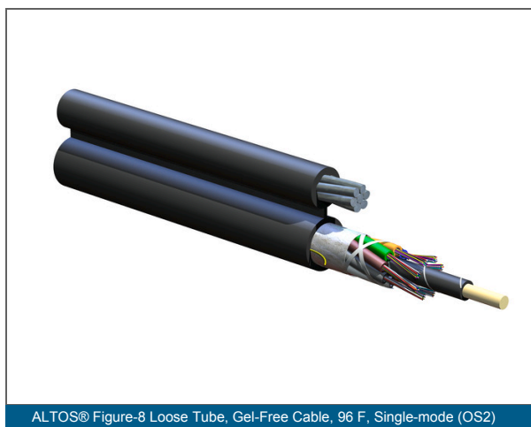
ALTOS® Figure-8 Loose Tube, Gel-Free Cable, 96 F, Single-mode (OS2)
