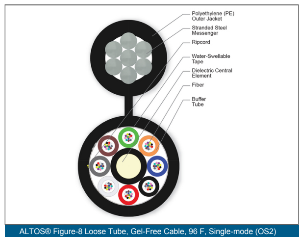
ALTOS® Figure-8 Loose Tube, Gel-Free Cable, 96 F, Single-mode (OS2)
